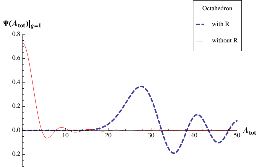
Figure 4: Wave Function \Psi versus total area for the octahedron lattice, with and without curvature contribution. The wave function is shown here for g = \sqrt{G} = 1 , a value chosen here for illustration purposes. The relevant expression for the wave function is given in Eq. (153). We refer to the text for further details on how the wave function was obtained, and what its domain of validity is. The wave functions shown here have been properly normalized. Note that with a nonzero curvature term the peak in the wave function moves away from the origin.
