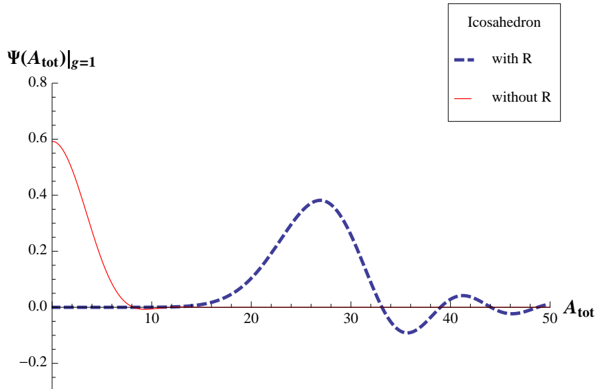
Figure 5: Same wave function \Psi as in Fig. 4, but now for the icosahedron lattice.
