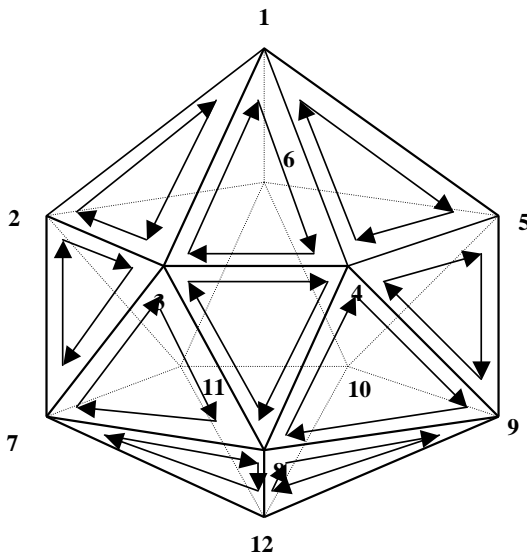
Fig 2. Elementary closed surface tiled with parallel transport polygons. For each link of the dual lattice, the parallel transport matrices \mathbf{R} are represented by an arrow. In spite of the fact that the Lorentz matrices \mathbf{R} fluctuate with the local geometry, two contiguous, oppositely oriented arrows always give \mathbf{R}\mathbf{R}^{-1} = 1 .
