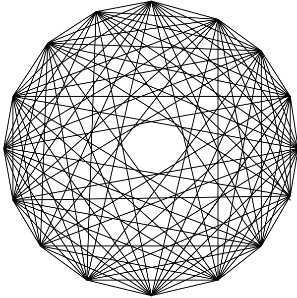
Fig 1. Cross polytope \beta_n with n = 8 and 2n = 16 vertices, whose surface can be used to define a simplicial manifold of dimension d = n - 1 = 7 . For general d , the cross polytope \beta_{d+1} will have 2(d + 1) vertices, connected to each other by 2d(d + 1) edges.
