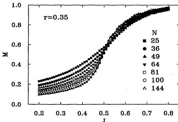
FIG. 9. The magnetization M versus J , for fixed hard-core repulsion parameter r = 0.35 and different system sizes. The solid line is a spline through the data for N = 144 .
