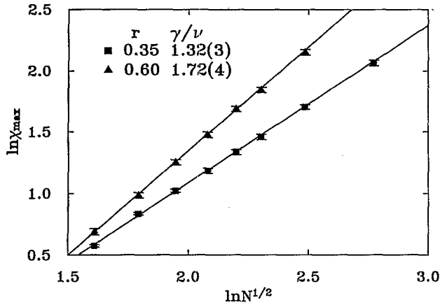
FIG. 8. The peak in the magnetic susceptibility \chi_{\max} versus the number of Ising spins N for choices of the hard-core repulsion parameter corresponding to r = 0.35 and r = 0.6 .
