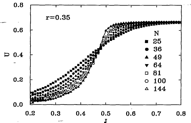
FIG. 14. The Binder fourth-order cumulant U as a function of J for fixed hard-core repulsion r = 0.35 and on several lattices with N spins. The solid line is a spline through the data for N = 144 .
