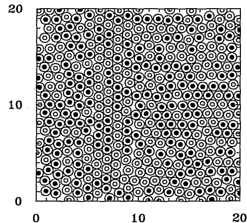
FIG. 3. A particular configuration of the system with N = 400 spins and r = 0.98 for J = 0.25 . The hard-core repulsion radius is shown as a circle around the spin. Spins with S = \pm 1 are indicated with open and solid circles, respectively.
