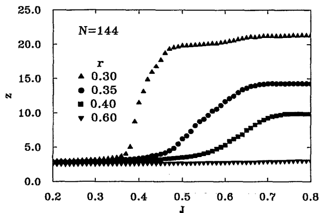
FIG. 4. The average number of neighbors z as a function of J on a lattice with N = 144 spins for several choices of the hard-core repulsion r .
