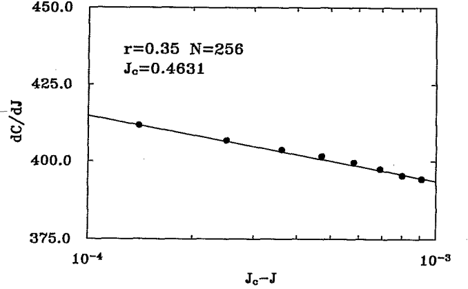
FIG. 13. The derivative of the specific heat dC/dJ as a function of J_c - J on semilogarithmic axes for N = 256 .
