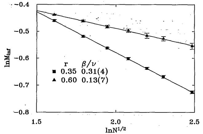
FIG. 10. Finite-size scaling of the magnetization at the inflection point M_{\text{inf}} versus the total number of Ising spins, N , for choices of the hard-core repulsion parameter corresponding to r = 0.35 and r = 0.6 .
