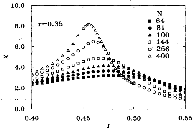
FIG. 7. The magnetic susceptibility \chi versus J for fixed hard-core repulsion parameter r = 0.35 and different system sizes.
