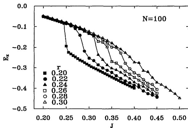
FIG. 5. The average energy per bond E_x as a function of J for several choices of the hard-core repulsion r for a system with N = 100 sites.
