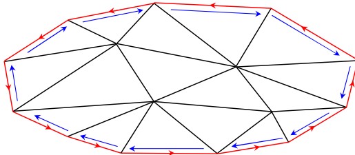
Figure 10. Illustration on how a perimeter contribution to the gravitational Wilson loop arises from matter field contributions. Note that now the arrows representing rotation matrices reside in principle in different representations.
