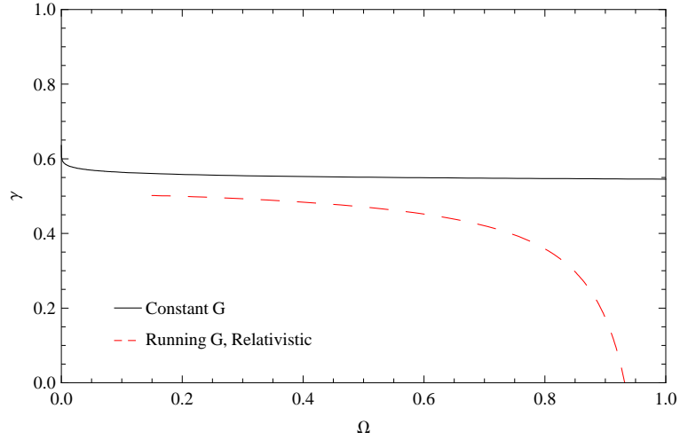
Figure 3. Illustration of the growth index parameter \gamma of Eq. (4.3) as a function of the matter density fraction \Omega , computed in the fully relativistic (tensor box) theory with a running G(a) as given in Eq. (3.11), and obtained by solving Eq. (3.75) with \gamma_\nu = 9/2 and c_a = 0.0003 . For the specific choice of matter fraction \Omega = 0.25 one then obtains the estimates given for the tensor box in Eq. (4.4). Not surprisingly the deviations from the standard result for \gamma become more visible for larger values of \Omega .
