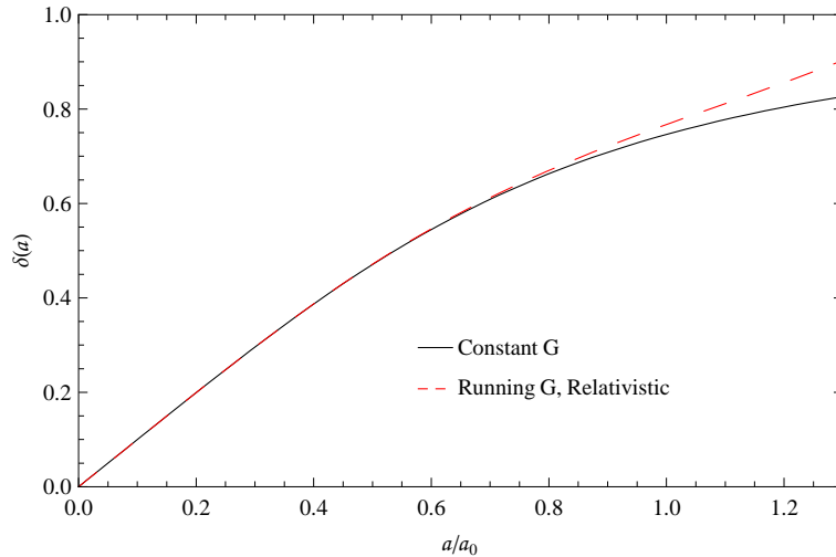
Figure 1. Illustration of the matter density contrast \delta(a) as a function of the scale factor a(t) , in the fully relativistic treatment (tensor box) and for a given matter fraction \Omega = 0.25 , obtained from the solution of the density contrast equation of Eq. (3.76), with G(a) given in Eq. (3.11) with \gamma_\nu = 9/2 and for c_a = 0.001 . In the case of a running G(\square) , one generally observes a slightly faster growth rate for later times, as compared to the solution for the case of constant G and with the same choice of \Omega , described by Eq. (3.87).
