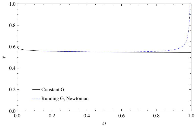
Figure 2. Illustration of the growth index parameter \gamma of Eq. (4.3) as a function of the matter density fraction \Omega , computed in the Newtonian (non-relativistic) theory with a running G(a) given in Eq. (3.11), and obtained by solving Eq. (A.36), here with \gamma_\nu = 9/2 and c_a = 0.01 . For the specific choice of matter fraction \Omega = 0.25 , suggested by \Lambda CDM models, one then obtains the estimates for the growth index parameter given in Eq. (4.6).
