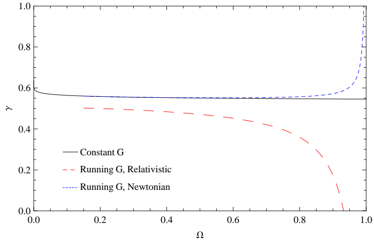
Figure 4. Qualitative comparison of the growth index parameters \gamma of Eq. (4.3) as a function of the matter density fraction \Omega , computed first in the relativistic (tensor box) theory with a running G(a) and c_a = 0.0003 , then in the Newtonian (non-relativistic) treatment also with a running G(a) and c_a = 0.01 , both with \gamma_\nu = 9/2 , and finally \gamma compared to the usual treatment with constant G . In both cases the deviations from the standard result for \gamma are most visible for larger values of \Omega , corresponding to a greater matter fraction.
